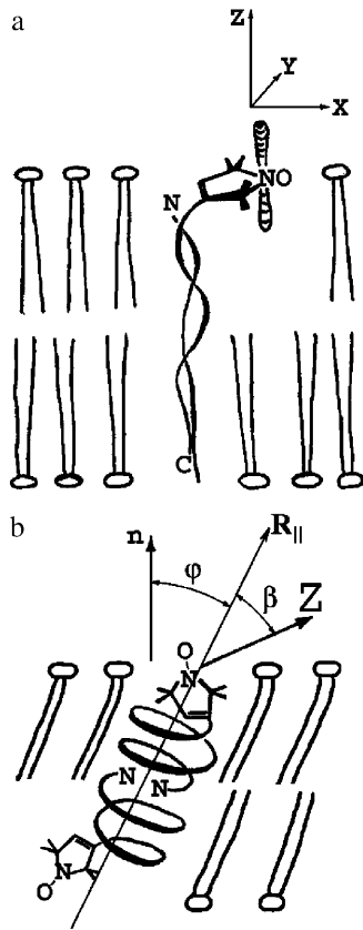
FIGURE 8 Schematic drawings of the conformations of GAsI in DMPC (a) and DPPC (b). For angles \beta and \phi , see text.
