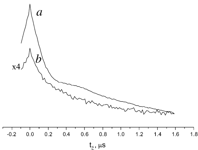
FIGURE 12 Time-domain DQC-ESR signals from GAsI/DPPC (0.12 mol %) samples. ( a ) A sample rapidly frozen from the L_\alpha phase; ( b ) a sample frozen from the L_\beta phase. Note that the smaller amplitude in case b is due to the property of DQC that it senses only the dipolar-modulated part of the spin-echo. There are fewer detectable nitroxide pairs in b as compared to a . The background signal is caused by intermolecular dipolar couplings (Borbat et al., 2002). A smaller background signal in b may be caused by a significant fraction of GA existing in the L_\beta phase in the form of small aggregates, leading to a rapid decay of the echo on the timescale required to acquire the signal from GAsI pairs.
