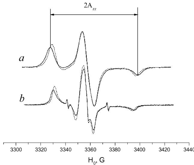
FIGURE 9 GAsI in DPPC (solid line) and DMPC (dashes) at 77 \text{ K} (a) and 10^\circ\text{C} (b). Molar ratio GAsI/lipid = 0.6\% .
