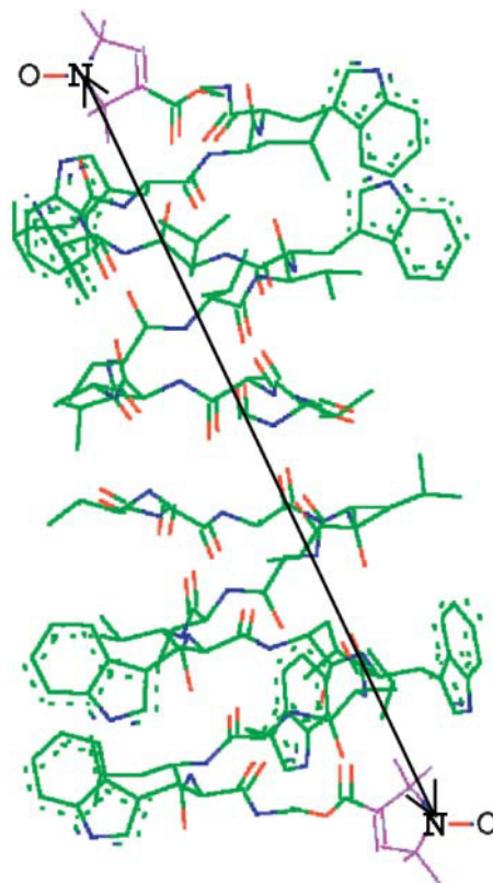
FIGURE 1 GAsl in the head-to-head conformation. The arrow indicates a distance of 29.5 Å between the nitroxide nitrogen atoms at the spin-labeling sites on the different C-termini of the dimer obtained from the structure for the GA channel given by Ketchum et al. (1997) and molecular modeling of the nitroxide tethers (see text).
